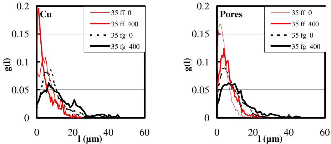
Fig. 3. Evolution with time of the chord lengths distribution of copper and pores for the mixtures 'ff' and 'fg', 35 vol% Cu ( g(l) denotes the length weighed chords distribution).
