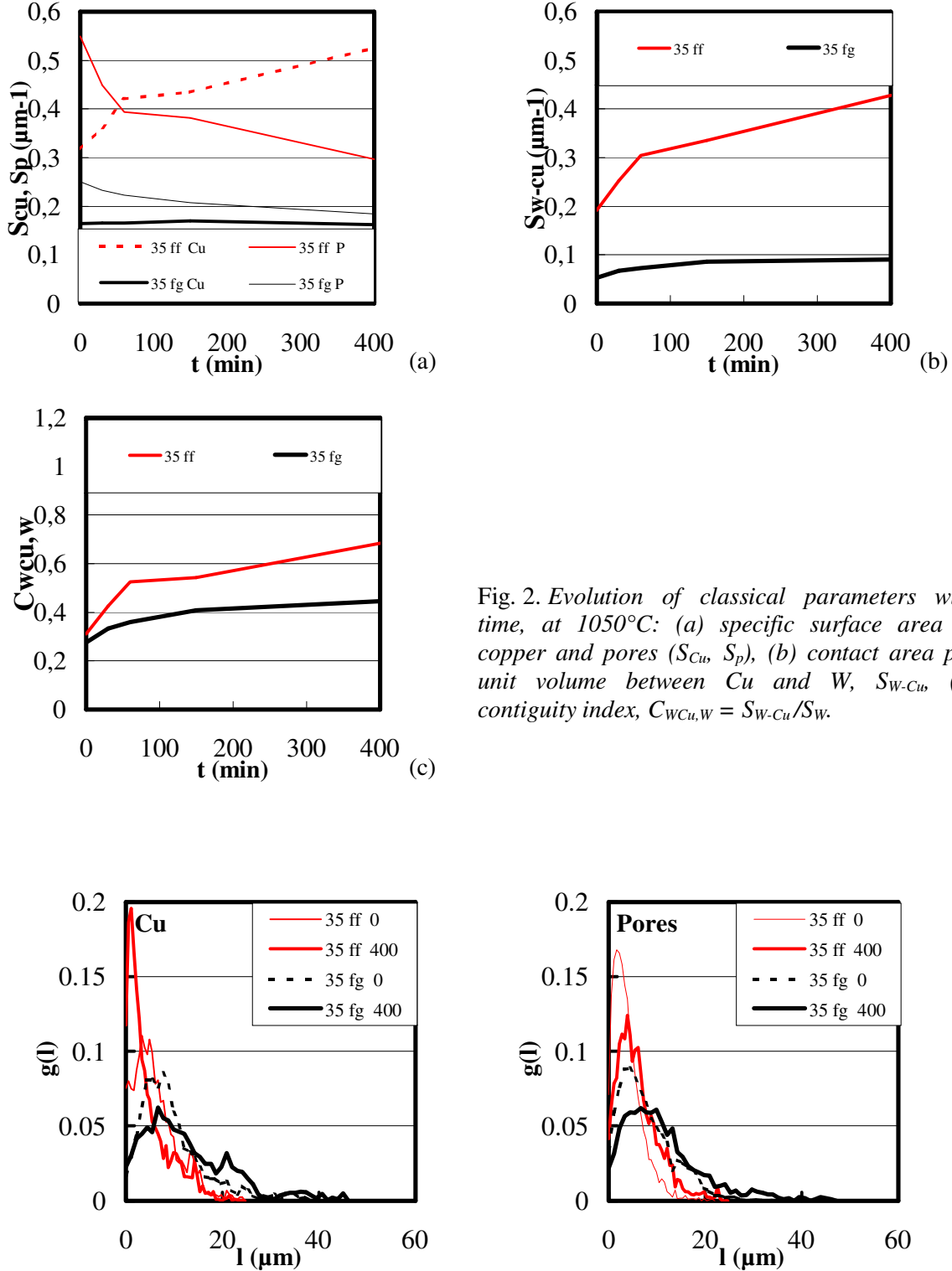
Fig. 3. Evolution with time of the chord lengths distribution of copper and pores for the mixtures 'ff' and 'fg', 35 vol% Cu ( g(l) denotes the length weighed chords distribution).
